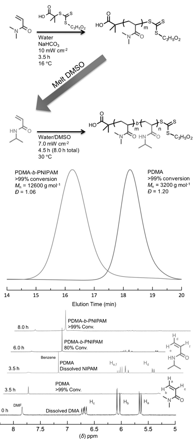
Figure 2. PDMA- b -PNIPAM was prepared in 8.0 h upon full monomer conversion of each block without the addition of an exogenous initiator. A clean shift in the molecular weight distribution is observed, indicative of good blocking efficacy. The 1 H NMR spectra highlight full monomer conversion of both DMA and NIPAM using DMF and benzene as internal standards, respectively.
